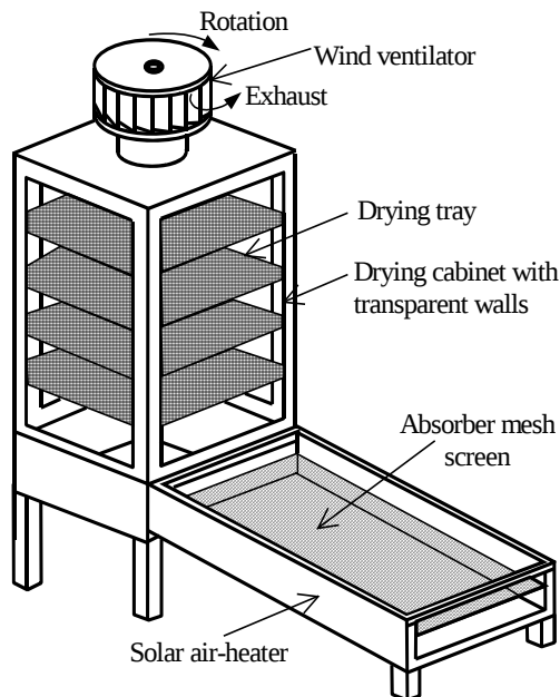
Figure 2. Solar wind-ventilated cabinet dryer
