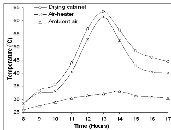
Figure 3. Diurnal variation of the temperatures in the solar dryer during the 1st day of the test
