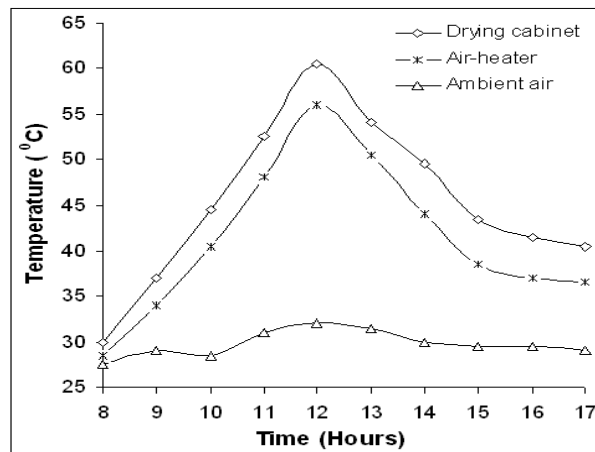
Figure 4. Diurnal variation of the temperatures in the solar dryer during the 2nd day of the test
